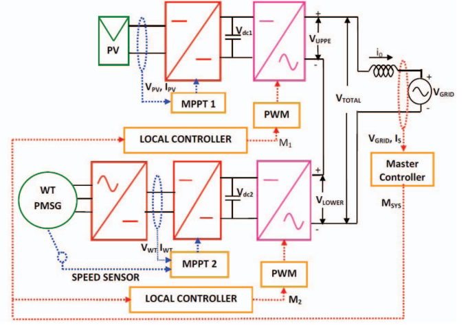
Fig. 7. Proposed Control System for cascaded MLI.
