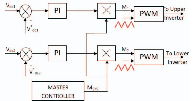
Fig. 9. Local Controllers.
